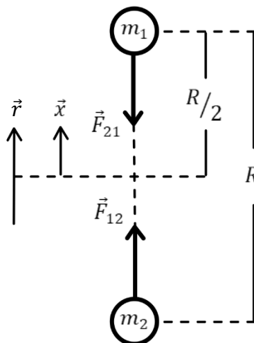
Figure 1: Two-Body Free-Fall
